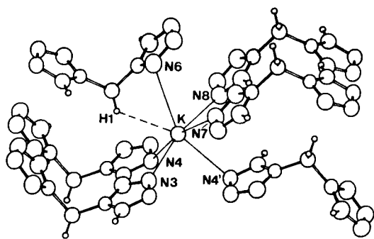
Fig. 2. Coordination sphere around potassium in 1 . Selected distances [pm] and angles [°]: K–N3 282.5(3), K–N4 290.3(3), K–N7 290.5(3), K–N8 291.4(3), K–N4' 292.7(2), K–N6 318.0(3), K⋯H 289.0(30), N4'–K–N6 149.23(7), N4'–K⋯H 153.3(6), N6–K⋯H 52.0(5), N3–K–N4' 87.73(8), N3–K–N4' 87.11(7), N7–K–N4' 80.86(8), N8–K–N4' 80.29(8); the angles in the equatorial plane lie between 88.05 and 90.85 (167.94(8) for the trans nitrogens).
