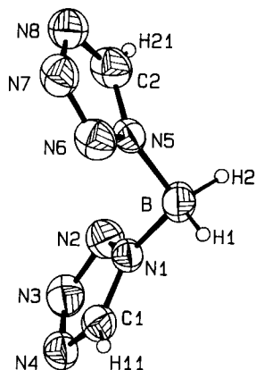
Fig. 1. Molecular structure of the [H_2B(CHN_4)_2]^- anion of 1 (ORTEP, 50% probability ellipsoids for non-hydrogen atoms; arbitrary radii for hydrogen atoms). Selected distances [pm] and angles [°]: B–N1 155.3(4), B–N5 156.1(4), B–H1 110(3), B–H2 109(3), N1–N2 134.0(3), N2–N3 129.6(3), N3–N4 134.5(3), N4–C1 131.6(4), C1–N1 131.9(4), N5–N6 134.2(3), N6–N7 130.1(3), N7–N8 134.2(3), N8–C2 130.0(4), C2–N5 131.8(4), N1–B–N5 109.1(3), B–N1–N2 122.7(3), B–N1–C1 130.6(3), N1–N2–N3 107.5(2), N2–N3–N4 110.3(2), N3–N4–C1 104.9(3), N4–C1–N1 110.5(3), C1–N1–N2 106.7(3); the respective angles in the other ring are very similar.
