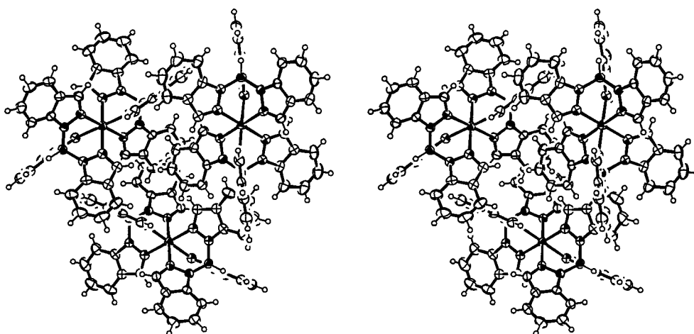
Figure 6. Stereoview of the section of the crystal structure of 4 \cdot 3.5 \text{CHCl}_3 (isostructural with 5 \cdot 3.5 \text{CHCl}_3 ) to illustrate the C–H... \pi interactions between the indazolyl moieties; solvent molecules have been omitted; view approximately along c
