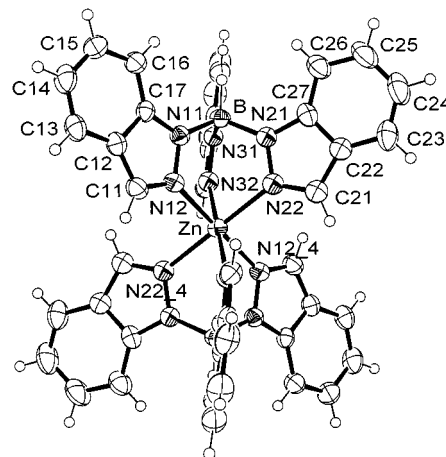
Figure 4. Molecular structure of [Zn{HB(C 7 H 5 N 2 ) 3 } 2 ] ( 8 ); selected distances [Å] and angles [°]: Zn–N12 2.157(3), Zn–N22 2.156(3), Zn–N32 2.149(3); N12–Zn–N22 84.0(1), N12–Zn–N32 86.4(1), N22–Zn–N32 87.2(1), N12–Zn–N22 4 96.1(1), N32–Zn–N12 4 93.7(1), N32–Zn–N22 4 92.9(1) (see also Table 4) (symmetry-equivalent position 4 = 1 – x, –y, 1 – z)
