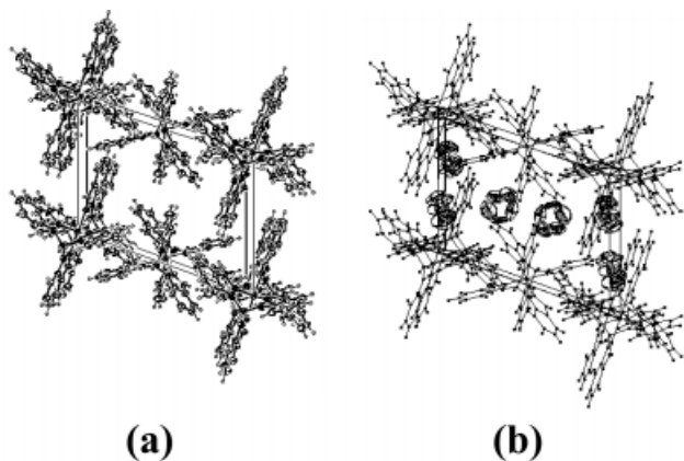
Figure 9. (a) Solvent-deleted crystal structure of 6 \cdot 3 THF showing the channel formation along a and (b) the same view with a wire-frame model of the metal complexes together with the THF molecules
