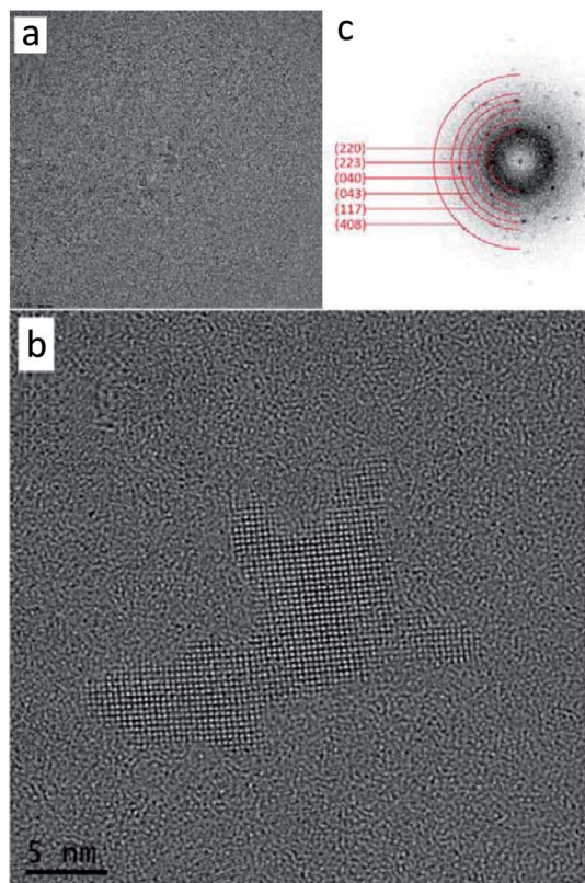
Fig. 6 (a) Overview TEM images of with the electron beam crystallized Fe/Al NPs (indicated by red arrow) in the IL [OPy][NTf 2 ]. (b) HRTEM of a single particle. (c) FFT of the NPs and the assignment based on the ICSD 151129 for (bulk) Fe 4 Al 13 .
